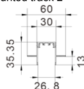
Recessed track
