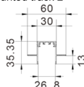
Recessed track
