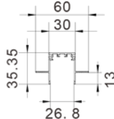
Recessed track
