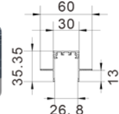
Recessed track
