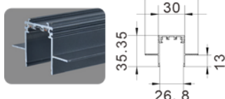
Recessed track
